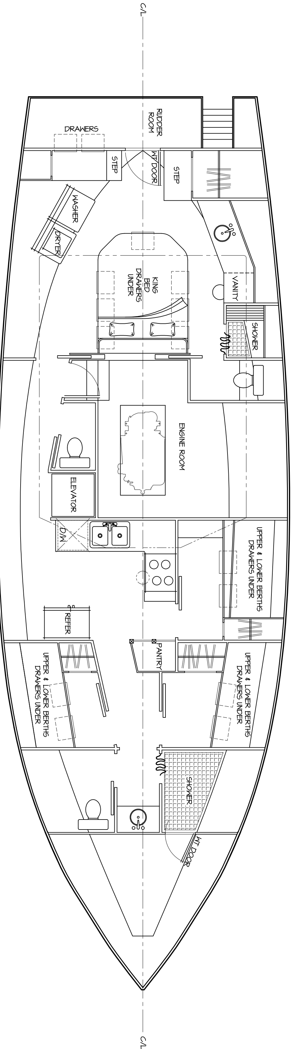
INTERIOR PLAN SCALE 1/4" = 1'-0"
