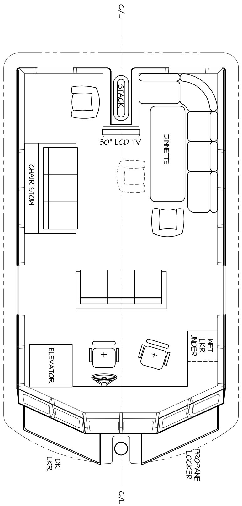
DECK HOUSE SCALE 1/4" = 1'-0"
